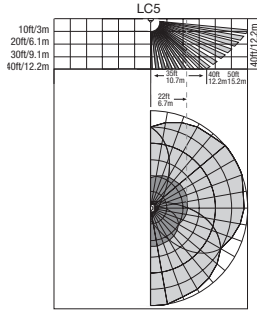
LC5 180° half moon lens cover for HBS 300 (347-480V)
