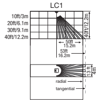
LC1 aisle starter cover for HBS 200 (347-480V)
