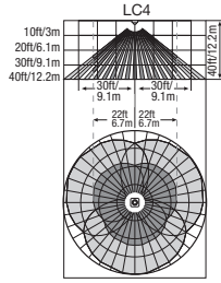
LC4 reduced range lens cover for HBS 300 (347-480V)
